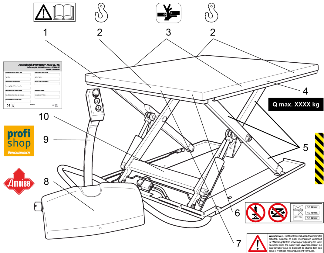
Fig. 3: Warning and information signs on the device
