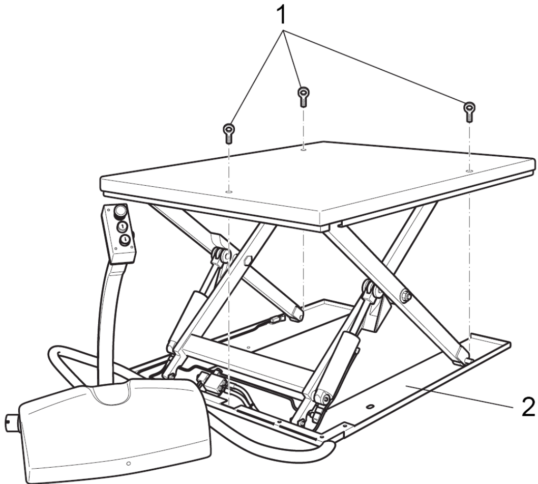
Fig. 6: Attachment points on lift table (example depiction)
