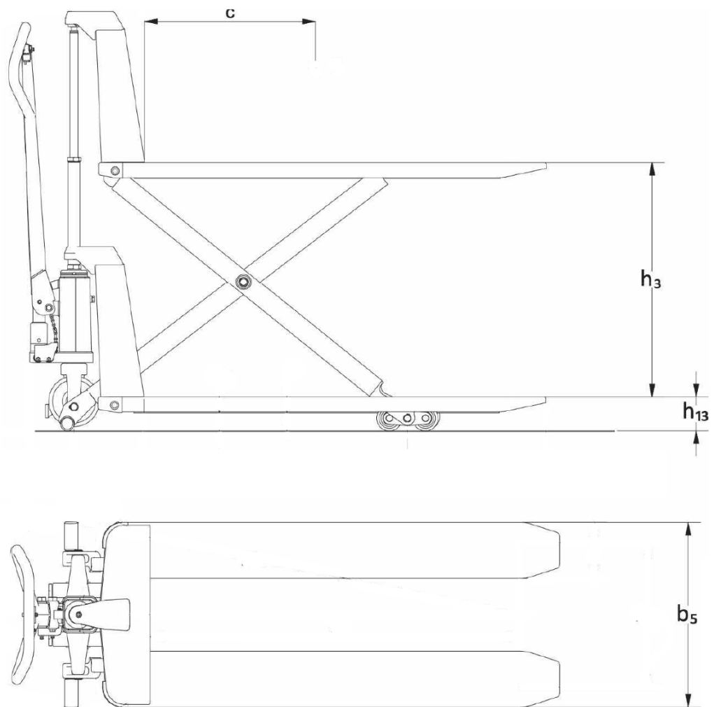
Fig. 3: Device dimensions (side view and top view, schematic)
