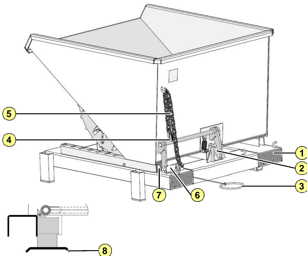
Fig. 3-1: Heavy Duty Tipper SK assemblies
