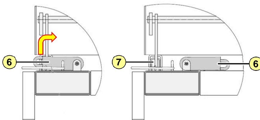
Fig. 5 5: Unlocking, option A
