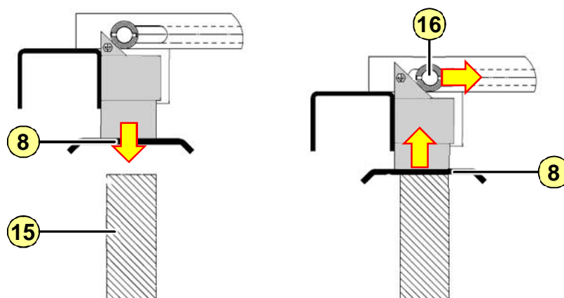
Fig. 5 6: Unlocking, option B
