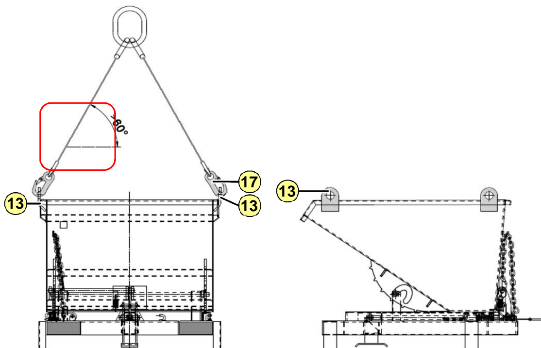
Fig. 5-8: Crane transport Heavy Duty Tipper
