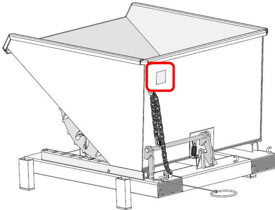
Fig. 2-2: Position of warning symbols/product safety labels
