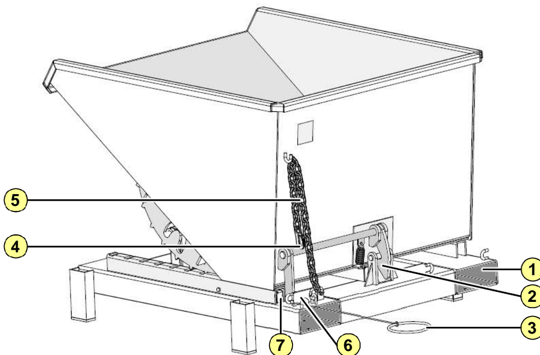
Fig. 5 2: Transport Heavy Duty Tipper
