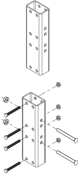
RR 80x50x4 x 275
