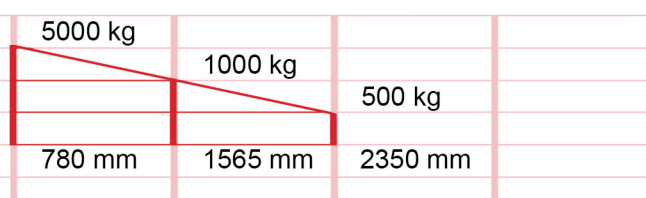
RLA-5 2400
