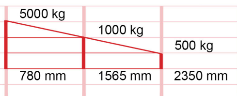
RLA-5 2400
