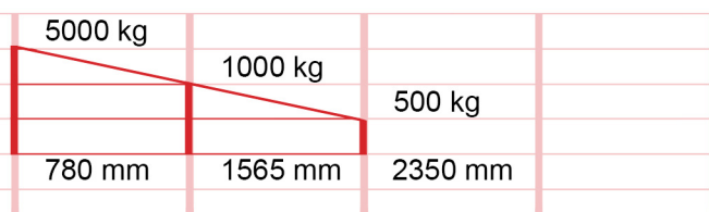
RLA-5 2400
