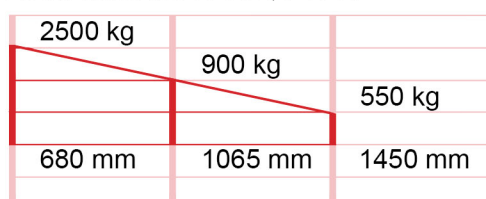
Load chart for RLA-2,5 1500
