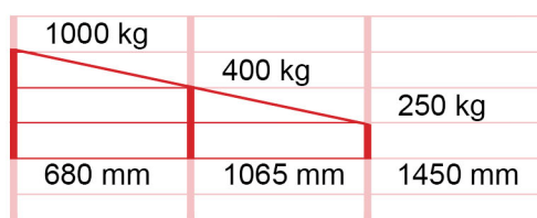
Load chart for RLA-1 1500
