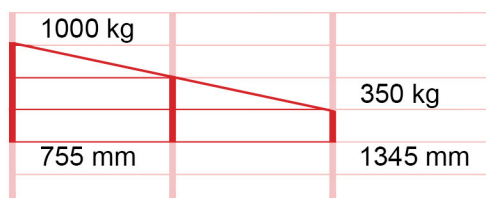
Load chart for RLH-1
